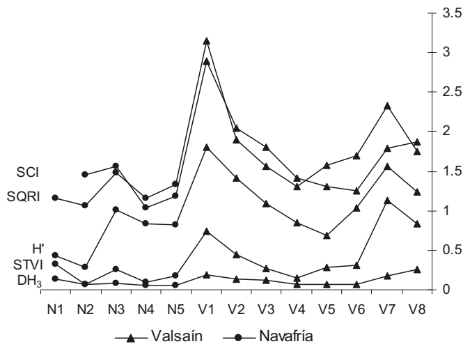
Figure 4. Value of the spatially and non-spatially explicit indices (SQRI, STVI, H', SCI and DH 3 ) in Valsain (V1–V8) and Navafria (N1–N5) forests.
