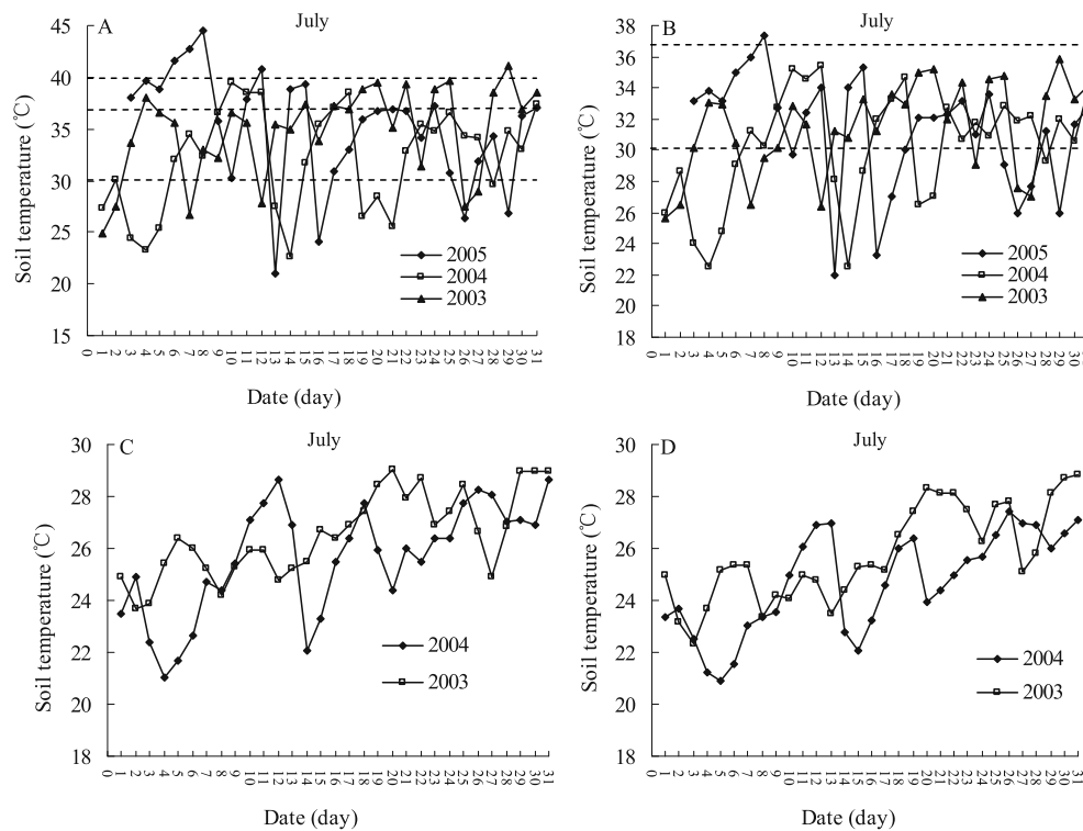
Figure 4. Soil temperature at experimental site: A: at 5 cm, B: at 10 cm, C: at 20 cm and D: at 40 cm (2003, 2004 and 2005). We present the temperature at 14:00 (GMT+08) in July because the annual maximum mean temperature appeared in July, and the daily maximum occurred at 14:00, which are important to the growth and survival of ECM.
